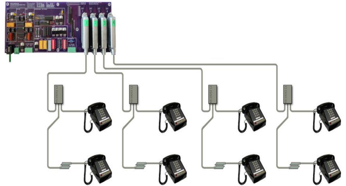
Fig. 56 – C-P-C connection blocks used to make extended chains of extensions.
